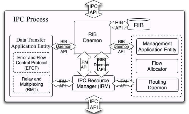
Fig. 3. RINA IPC process components and APIs
